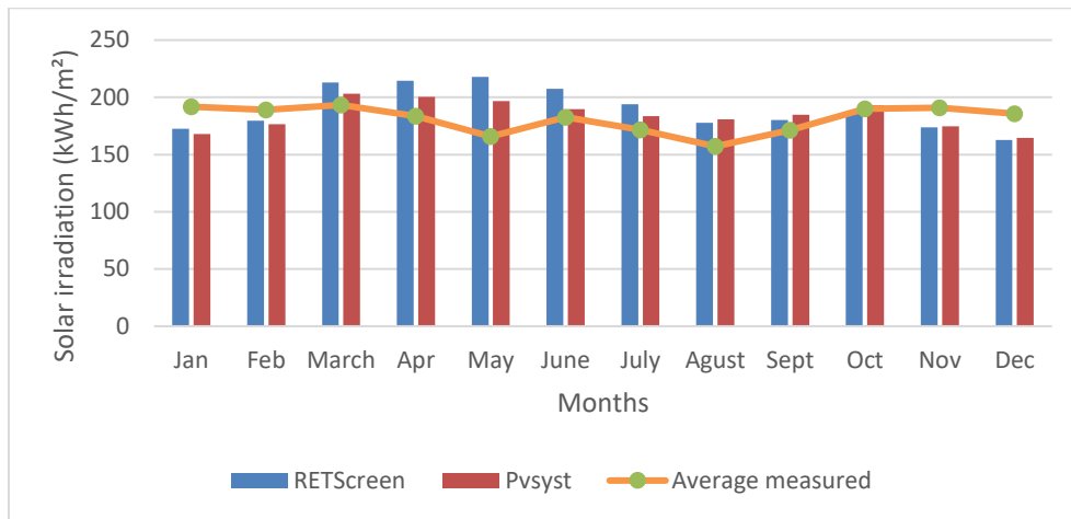
Fig. 1. Simulated monthly irradiance and average irradiance measured from 2019 to 2021
