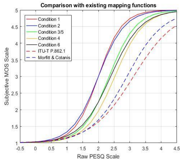
Fig. 4. Comparison of conditioned logistic functions with existing ones
