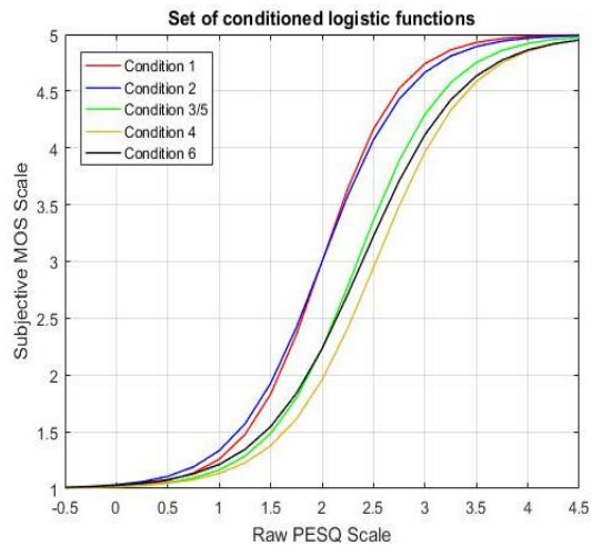
Fig. 3. Plot of logistic mapping functions as conditioned
