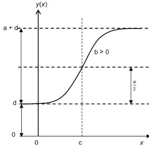
Fig. 2. Parameters of the offset logistic Growth function.
