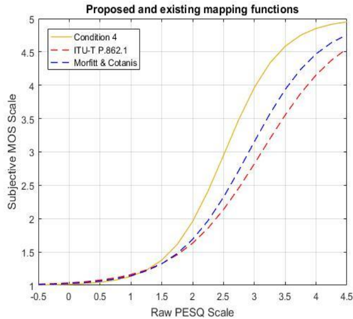
Fig. 6. Comparison of proposed logistic functions with existing ones
