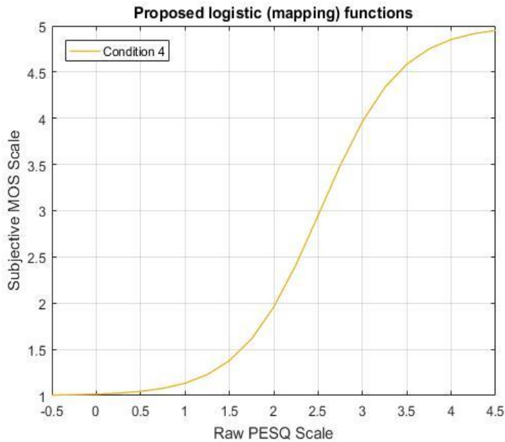
Fig. 5. Plot of proposed logistic function
