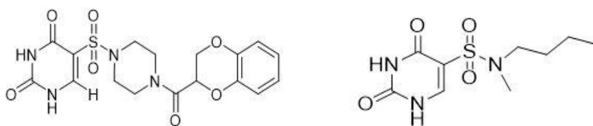
Fig. 1. Input structure of 5-(4-(2,3-dihydrobenzo[b][1,4]dioxine-2-carbonyl)piperazin-1-yl)sulfonylpyrimidine-2,4(1H,3H)-dione and N-butyl-N-methyl-2,4-dioxo-1,2,3,4-tetrahydro pyrimidine-5-sulfonamide
