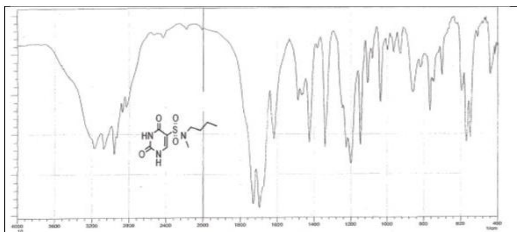
Fig. 3. Experimental and Theoretical FT-IR spectra of 5-(4-(2,3-dihydrobenzo[b][1,4]dioxine-2-carbonyl)piperazin-1-yl)sulfonyl)pyrimidine-2,4(1H,3H)-dione
