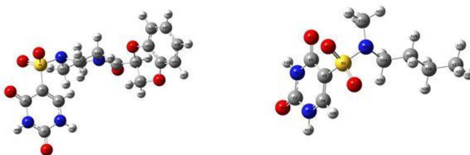
Fig. 2. The optimized geometrical structure of 5-(4-(2,3-dihydrobenzo[b][1,4]dioxine-2-carbonyl)piperazin-1-yl)sulfonyl)pyrimidine-2,4(1H,3H)-dione and N-butyl-N-methyl-2,4-dioxo-1,2,3,4-tetrahydropyrimidine-5-sulfonamide in solvent phase
