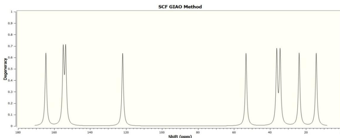
Fig. 8. Computational ^{13}\text{C} NMR spectra of N-butyl-N-methyl-2, 4-dioxo-1, 2, 3, 4-tetrahydropyrimidine-5-sulfonamide
