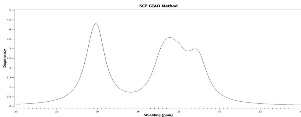
Fig. 9. Computational ^1\text{H} NMR spectra of 5-(4-(2,3-dihydrobenzo[b][1,4]dioxine-2-carbonyl)piperazin-1-yl)sulfonyl)pyrimidine-2,4(1H,3H)-dione
