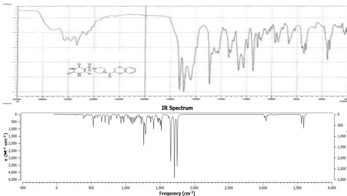
Fig. 3. Experimental and Theoretical FT-IR spectra of 5-(4-(2,3-dihydrobenzo[b][1,4]dioxine-2-carbonyl)piperazin-1-yl)sulfonyl)pyrimidine-2,4(1H,3H)-dione
