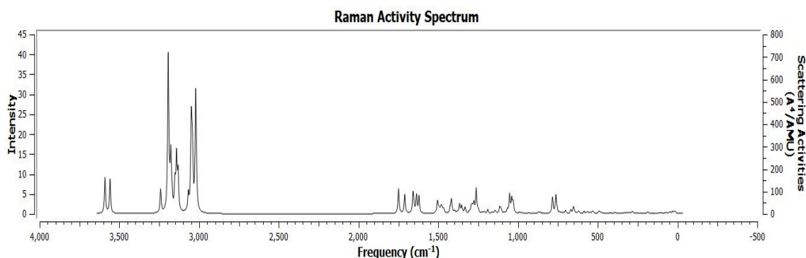
Fig. 5. Computational Raman spectra of 5-(4-(2,3-dihydrobenzo[b][1,4]dioxine-2-carbonyl)piperazin-1-yl)sulfonyl)pyrimidine-2,4(1H,3H)-dione
