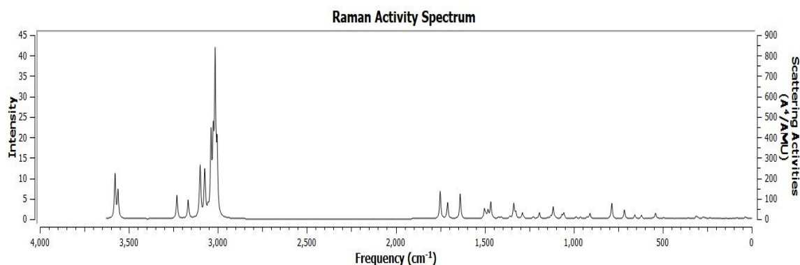
Fig. 6. Computational Raman spectra of N-butyl-N-methyl-2, 4-dioxo-1, 2, 3, 4-tetrahydropyrimidine-5-sulfonamide
