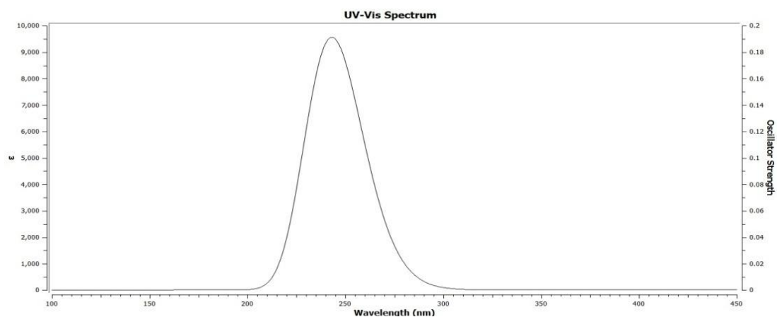
Fig. 11. Computational UV-Vis spectra of 5-(4-(2,3-dihydrobenzo[b][1,4]dioxine-2-carbonyl)piperazin-1-yl)sulfonyl)pyrimidine-2,4(1H,3H)-dione
