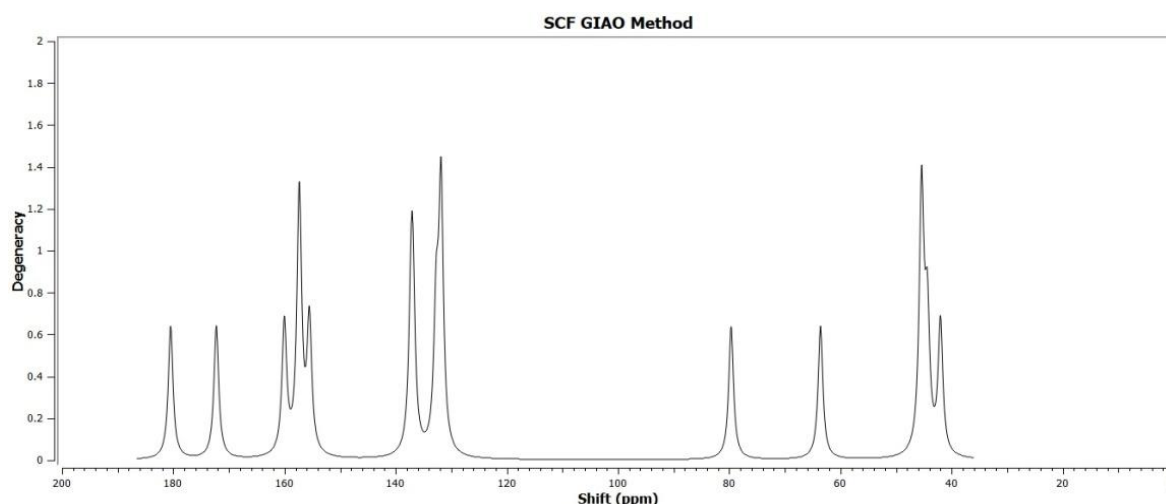
Fig. 7. Computational ^{13}\text{C} NMR spectra of 5-(4-(2,3-dihydrobenzo[b][1,4]dioxine-2-carbonyl)piperazin-1-yl)sulfonyl)pyrimidine-2,4(1H,3H)-dione
