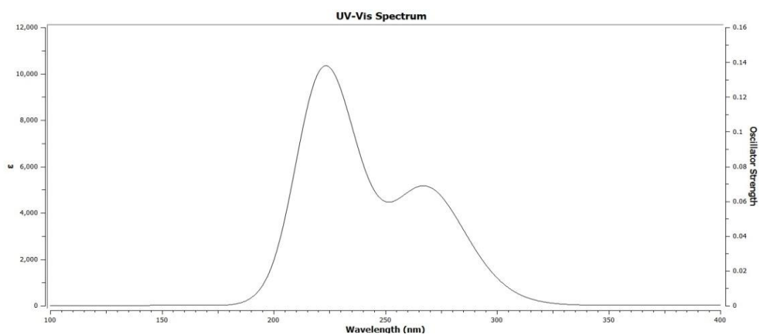
Fig. 12. Computational UV-Vis spectra of N-butyl-N-methyl-2,4-dioxo-1,2,3,4-tetrahydropyrimidine-5-sulfonamide
