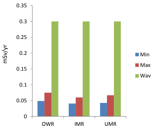
Fig. 3. Bar chart comparing the maximum (Max) and minimum (Min) values of AGDE with world average value (Wav) for the three surveyed rivers
