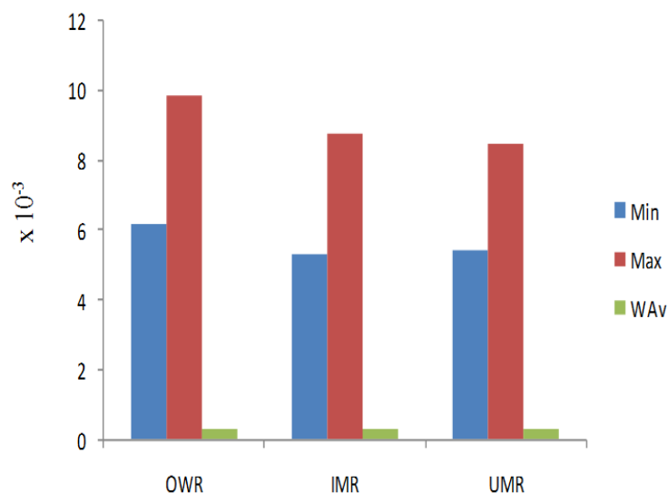
Fig. 4. Bar chart comparing the maximum (Max) and minimum (Min) values of ELCR with world average value (Wav) for the three surveyed rivers
