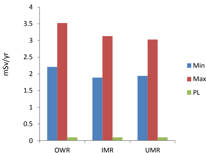
Fig. 2. Bar chart comparing the maximum (Max) and minimum (Min) values of EDIW with permissible limit (PL) for the three surveyed rivers
