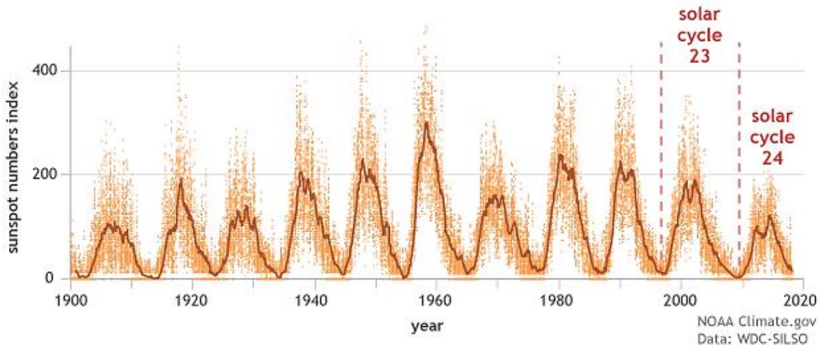
Solar activity over the past 11 sunspot cycles
