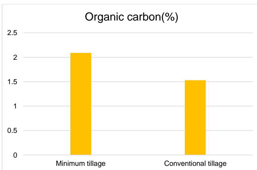
Fig. 4. Effect of tillage method on organic carbon content in the post- harvest soil, per cent
