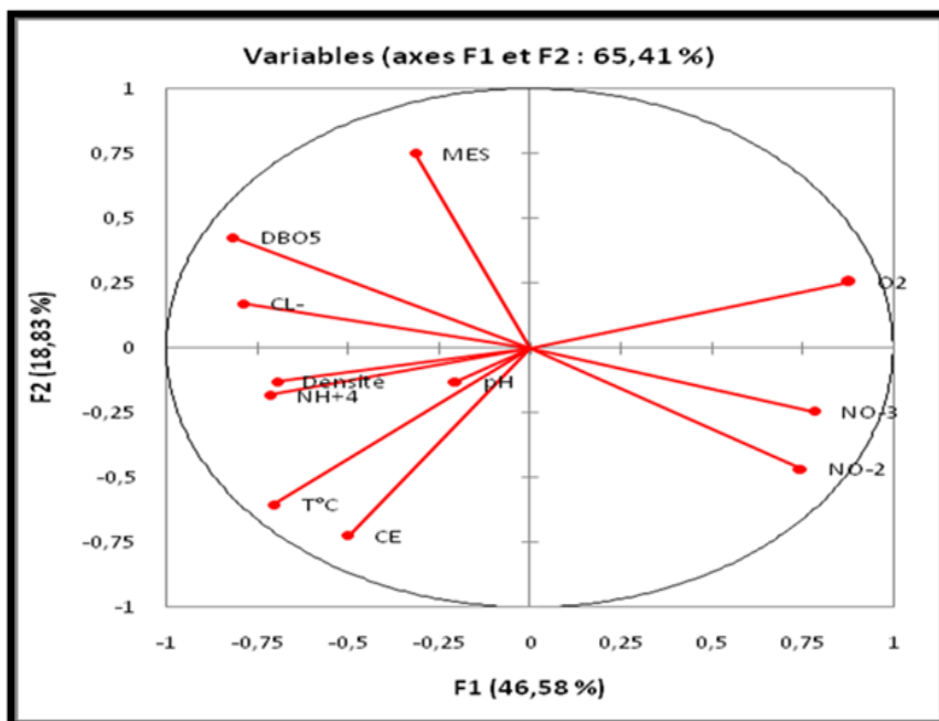
Fig. 3. Projection of variables into the space of factorial axes (F1 and F2)
