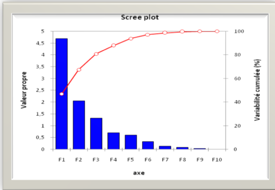
Fig. 2. Graphical representation of eigenvalue and cumulative variability
