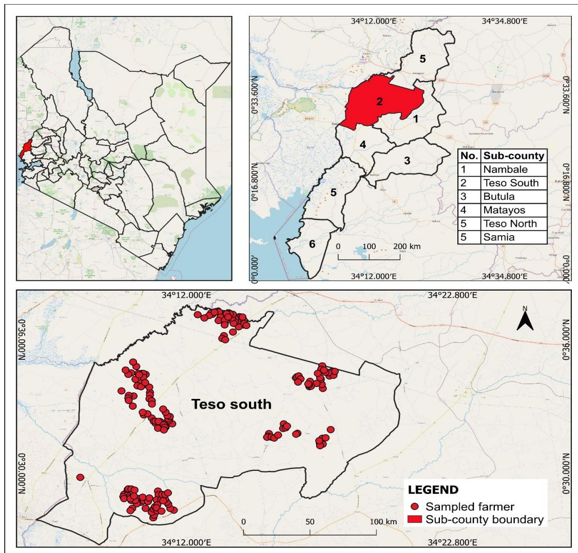
Fig. 1. Map of Busia County Showing study sites and sampled households
