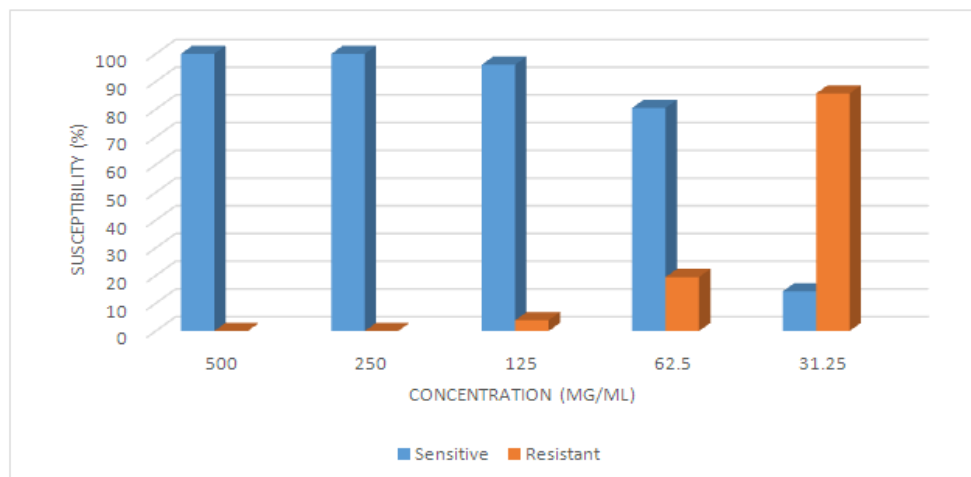
Fig. 1. Antibacterial activities of cocoa pod husk against Pseudomonas aeruginosa
