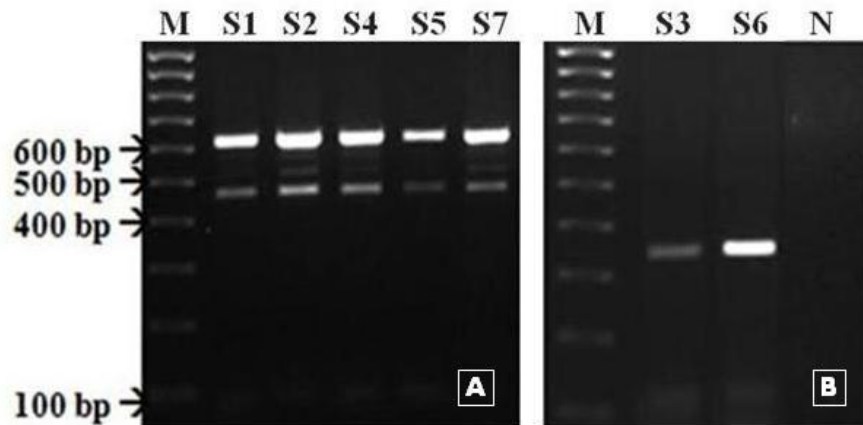
Fig. 1. Sequence-tagged Sites (STS) SSU rDNA primer-based PCR analysis of Blastocystis sp. subtypes of positive samples from symptomatic patients (S1-S5) and asymptomatic individuals (S6 and S7) using: SB227 (ST3-526bp), SB228 (ST3-473bp), and SB229 (ST3-631bp) combined primer pairs as a multiplex reaction for ST3 subtype (Panel A), and SB83 (ST1-351bp) primer pair for ST1 subtype detection (Panel B). Negative control (lane N) and 100 bp molecular size marker (lane M) separated in parallel
