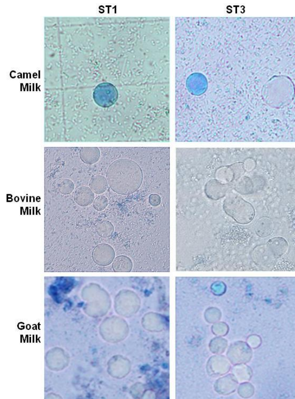
Fig. 2. ST1 and ST3 Blastocystis sp. parasites counting in haemocytometer (improved Neubauer chamber) after 48 h culture incubation in presence of 62.5 µl/ml of camel, bovine, and goat raw milks
