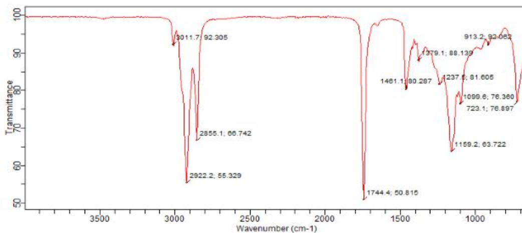
Fig. 2. FTIR spectrum for CSO extract
