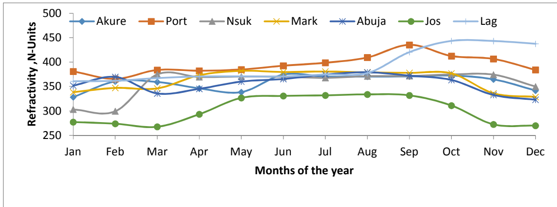
Fig. 8. Seasonal variation of surface refractivity over the stations for year 2011
