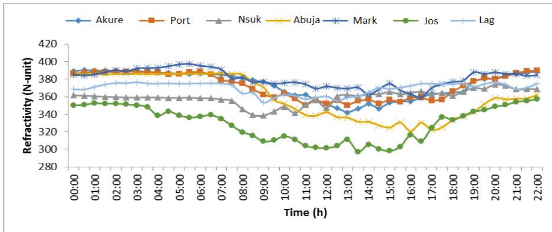
Fig. 4. Diurnal variation of surface refractivity for a typical day (1 st June) in wet season over all the stations for the year 2011
