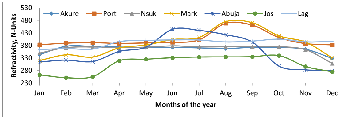
Fig. 9. Seasonal variation of surface refractivity over the stations for year 2012
