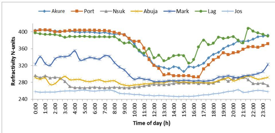
Fig. 7. Diurnal variation of surface refractivity for a typical day (1 st January) in dry season over all the stations for the year 2012
