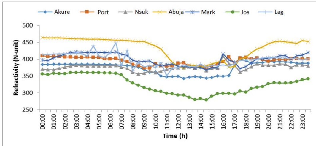
Fig. 5. Diurnal variation of surface refractivity for a typical day (1 st June) in wet season over all the stations for the year 2012
