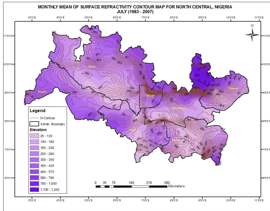
Fig. 4. Spatial patterns of surface refractivity with elevation in July (1983-2007) at North Central, Nigeria
