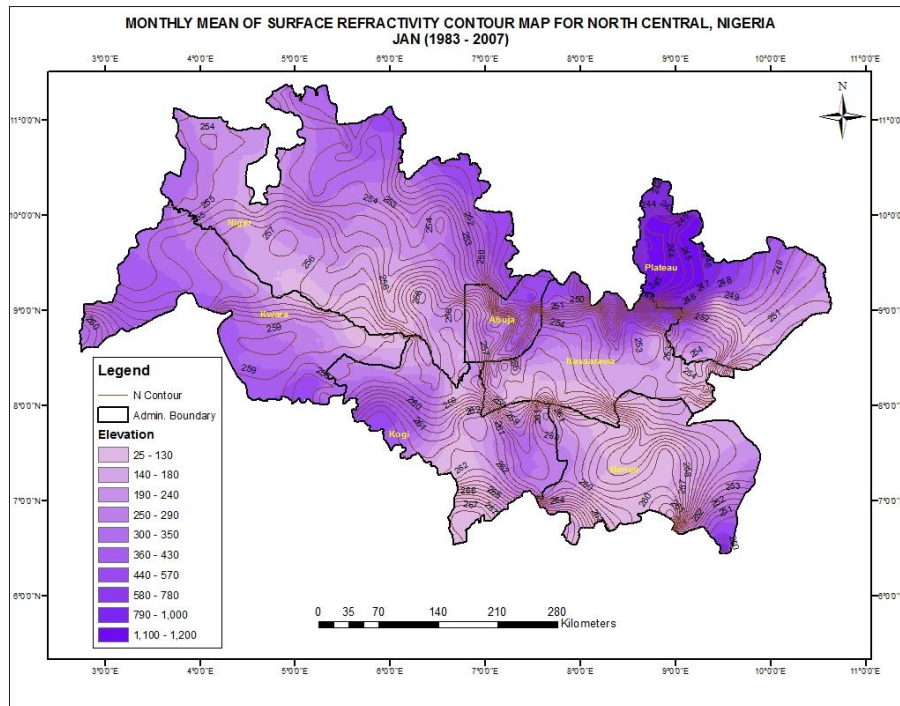
Fig. 3. Spatial patterns of surface refractivity with elevation in January (1983-2007) at North Central, Nigeria
