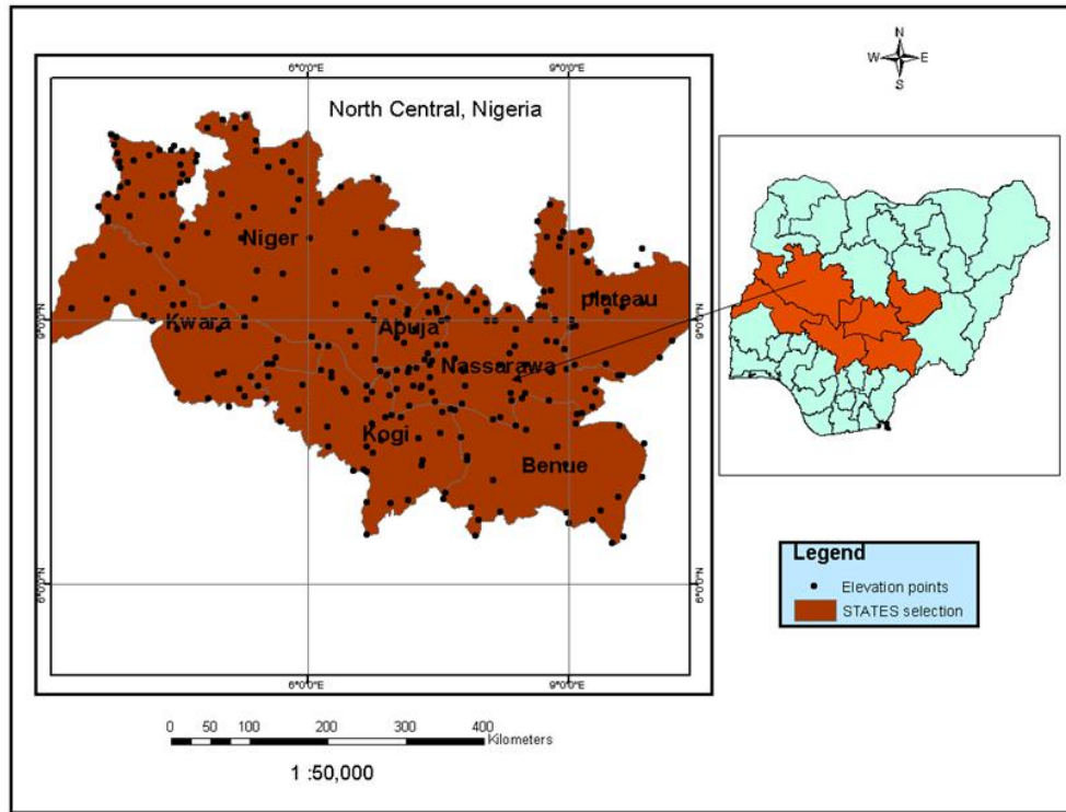
Fig. 1. Thematic map of North Central, Nigeria
