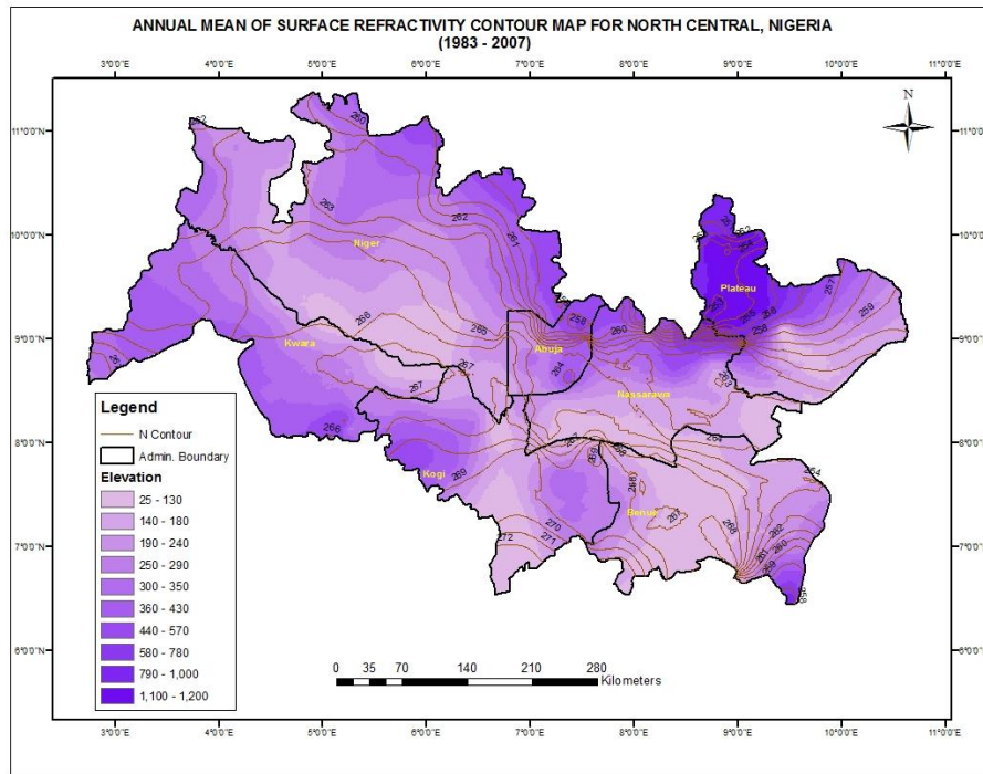
Fig. 2. Spatial patterns of annual surface refractivity with elevation (1983-2007) at North Central, Nigeria
