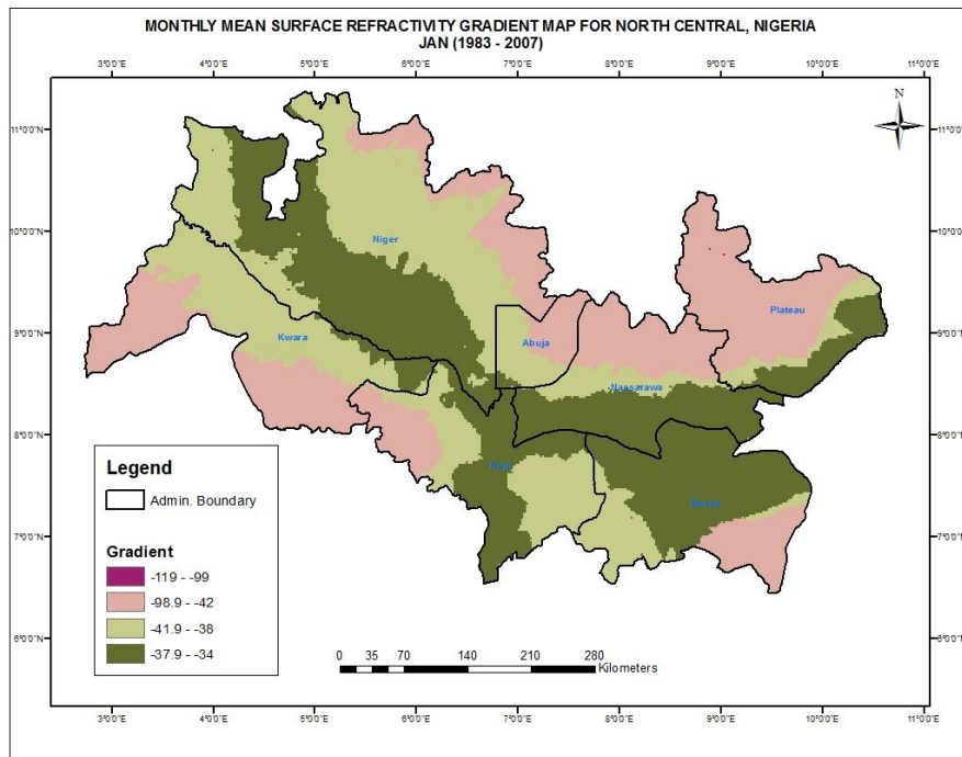
Fig. 6. Monthly mean of refractivity gradient patterns in January (1983-2007) at North Central, Nigeria
