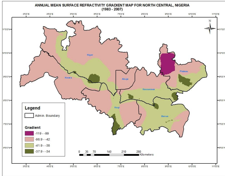
Fig. 5. Annual mean of refractivity gradient patterns (1983-2007) at North Central, Nigeria
